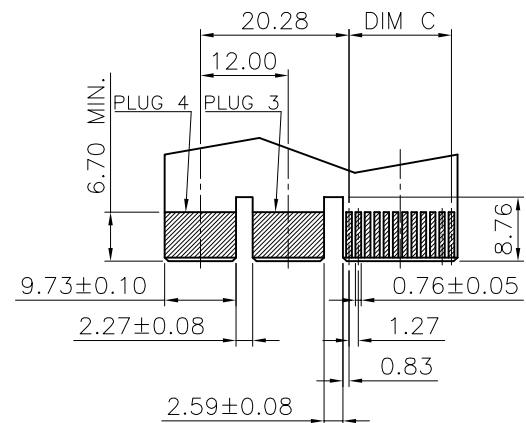
RECOMMENDED CARD EDGE LAYOUT
