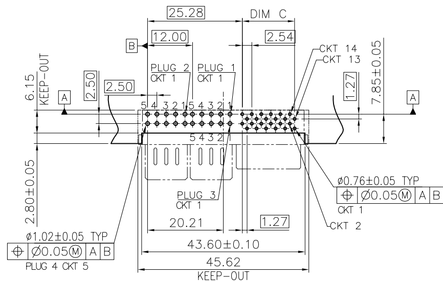
RECOMMENDED PCB LAYOUT COMPONENT SIDE
